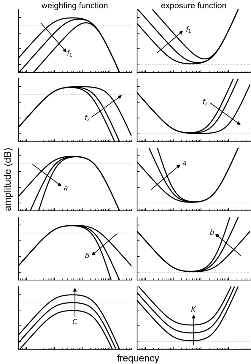
Figure A.2. Influence of parameter values on the resulting shapes of the weighting functions (left) and exposure functions (right). The arrows indicate the direction of change when the designated parameter is increased.
